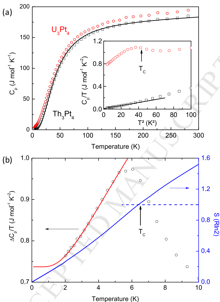
Figure 4. (a) Temperature dependence of the specific heat of \text{U}_3\text{Pt}_4 (open red circle) and its phonon counterpart \text{Th}_3\text{Pt}_4 (open black squares). The solid line corresponds to the fit of eq. (2) to the \text{Th}_3\text{Pt}_4 data. The inset presents the low temperature region of C_p/T as a function of T^2 for both compounds, the solid line being the fit of equation (3) to the \text{Th}_3\text{Pt}_4 data. (b) Low temperature variation of the 5f electron specific heat (open circles) and corresponding entropy (blue line) normalized to R \ln 2 values. The red solid line corresponds to the fit of equation (4) to the experimental \Delta C_p/T data. The horizontal dashed blue line indicates the R \ln 2 value of the entropy.
