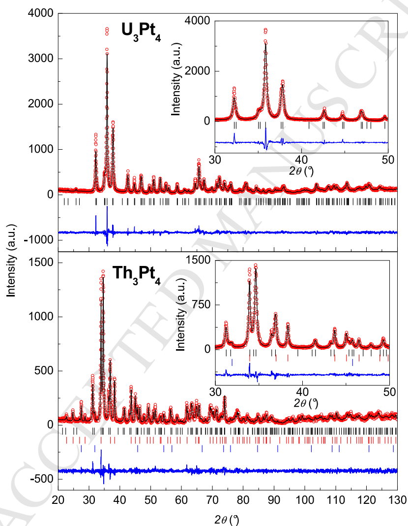
Figure 1. Rietveld refined X-ray diffraction patterns of \text{U}_3\text{Pt}_4 (upper panel) and \text{Th}_3\text{Pt}_4 (lower panel). The experimental data (red symbols), the calculated patterns (black line) and the difference between them (blue line) are presented. The vertical ticks represent the refined positions of the diffraction peaks of A_3Pt_4 ( A = \text{U}, \text{Th} ; black), \text{Th}_3\text{Pt}_5 (red) and \text{ThO}_2 (blue). The insets show zoomed areas of the main panel.
