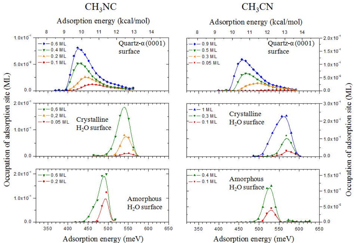
Fig. 6. Adsorption energy distributions for several initial submonolayer coverages of CH 3 NC (left) and CH 3 CN (right) adsorbed on \alpha -quartz (0001), crystalline water, and compact amorphous water surfaces.
