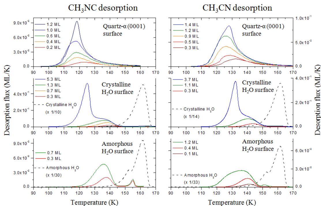
Fig. 4. TPD curves of several initial coverages of \text{CH}_3\text{NC} (left) and \text{CH}_3\text{CN} (right) adsorbed on \alpha -quartz (0001) surface, and on crystalline and compact amorphous water ice surface. Applied heating rates are 12 \text{ K min}^{-1} on quartz, and 10 \text{ K min}^{-1} on water surfaces. TPD curves of multilayers ( \approx 50 \text{ ML} ) of crystalline and amorphous water ice are shown in dashed lines for comparison.
