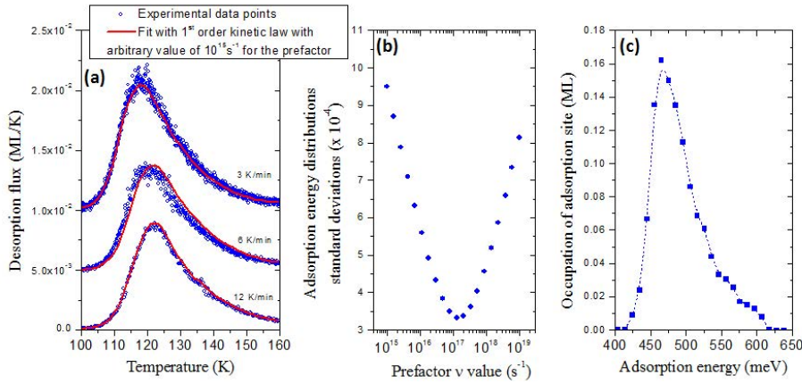
Fig. 5. a) Set of TPD curves of 0.2 ML of CH 3 CN adsorbed on \alpha -quartz (0001) performed at 3 K min -1 , 6 K min -1 , and 12 K min -1 . Straight lines are the fit of these data using a first order kinetic Polanyi-Wigner law with a distribution of adsorption energy using a prefactor of 10 15 s -1 . b) Search for the best value for the prefactor \nu : plot of the standard deviation of the three minimum occupied adsorption energies as extracted from the fits of the three TPD curves. The minimum of the curve give the best choice for \nu . c) Adsorption energy distribution corresponding to 0.2 ML of CH 3 CN on quartz using the best choice for the prefactor.
