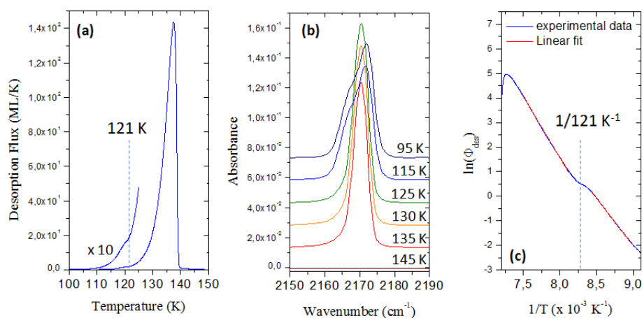
Fig. 2. a) TPD curve, with a heating rate of 2 \text{ K min}^{-1} , of \sim 800 \text{ ML} of pure \text{CH}_3\text{NC} deposited on polycrystalline gold at 90 \text{ K} . The beginning of the desorption has been magnified by a factor of 10. b) Infrared spectra in the region of the NC stretching vibration, during the warming up of the ice. c) Plot of the logarithm of the desorption flux as a function of the inverse of the temperature. Lines are linear fits of the plot.
