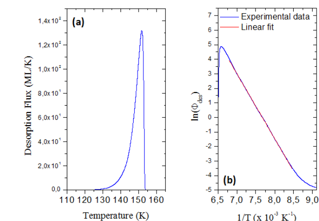
Fig. 3. a) TPD curve, with a heating rate of 2 \text{ K min}^{-1} , of \sim 800 \text{ ML} of pure \text{CH}_3\text{CN} deposited on polycrystalline gold at 90 \text{ K} . b) Plot of the logarithm of the desorption flux as a function of the inverse of the temperature.
