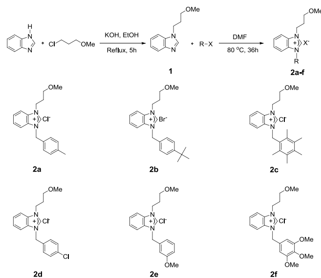
Scheme 2. Synthesis of the benzimidazolium salts ( 2a-f ).
