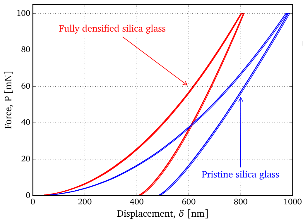
Figure 2. Nano-indentation force-displacements curves for pristine silica glass and fully densified silica glass. Five tests are carried out for each type, and experimental reproducibility is confirmed.
