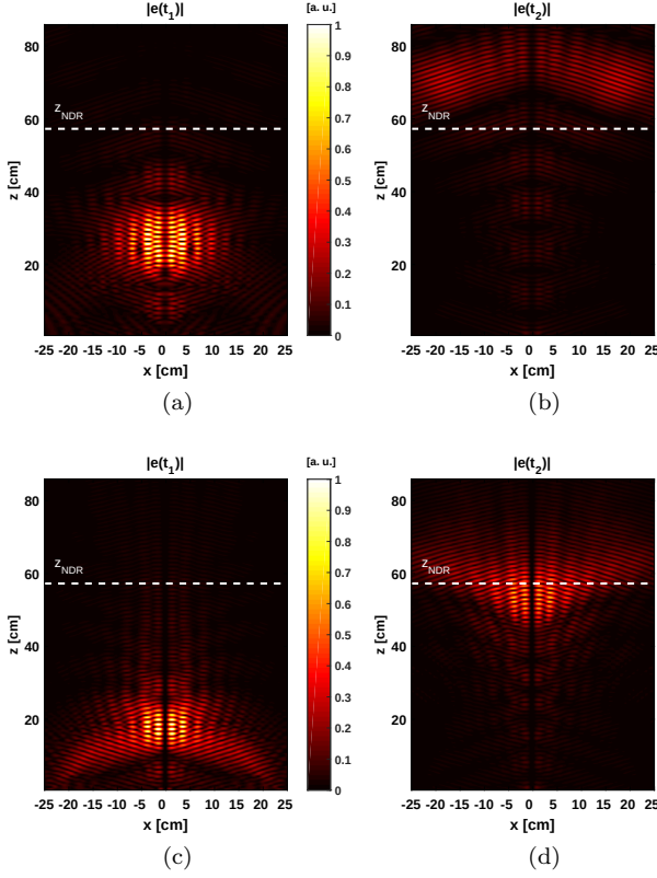
FIG. 3. XOAM field amplitude in the azimuthal xz ( \phi = 0 ) plane. Comparison between (a)-(b) nondispersive and (c)-(d) dispersive case. The intensity of the vectorial electric field |e| has been reported for two time instants: (a), (c) t_1 = 0.8 ns and (b), (d) t_2 = 2.4 ns. Note that t_1 and t_2 correspond to the time instants for which the nondispersive pulse would have traveled a distance equal to \frac{1}{2}z_{\text{NDR}} and \frac{3}{2}z_{\text{NDR}} , respectively (Multimedia view). Note that z_{\text{NDR}} = 57.3 cm
