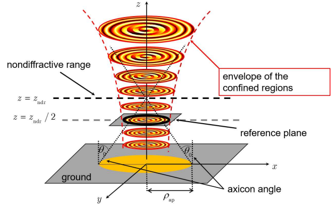
FIG. 1. Circular aperture over the xy plane for launching localized waves at microwaves. Their section slowly increases beyond the nondiffractive range due to the limited spatio-temporal dispersion of the pulse. A transverse reference plane at z_0 = z_{\text{NDR}}/2 is defined to observe the pulse propagation.
