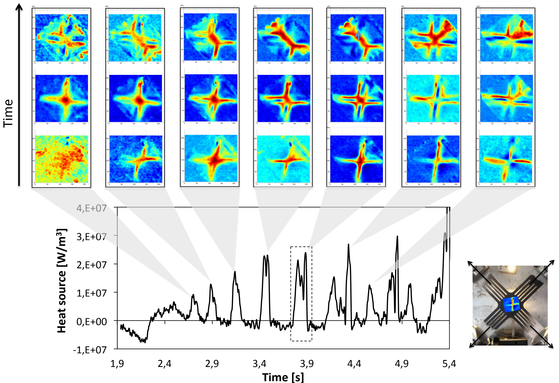
Figure 8: heat source maps highlight that the PLC band kinematic is the same. A double PLC band network is observed, especially at the highest strains
