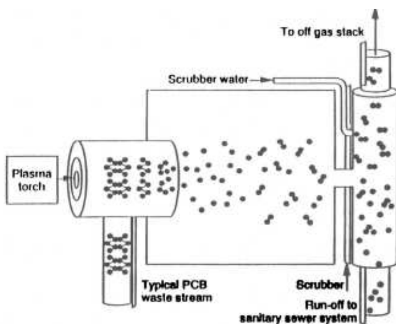
Fig. 14 Schematic diagram of pyrolysis unit for waste treatment.
