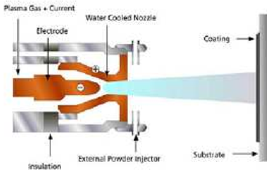
Fig 15 A schematic diagram of thermal plasma coating.
