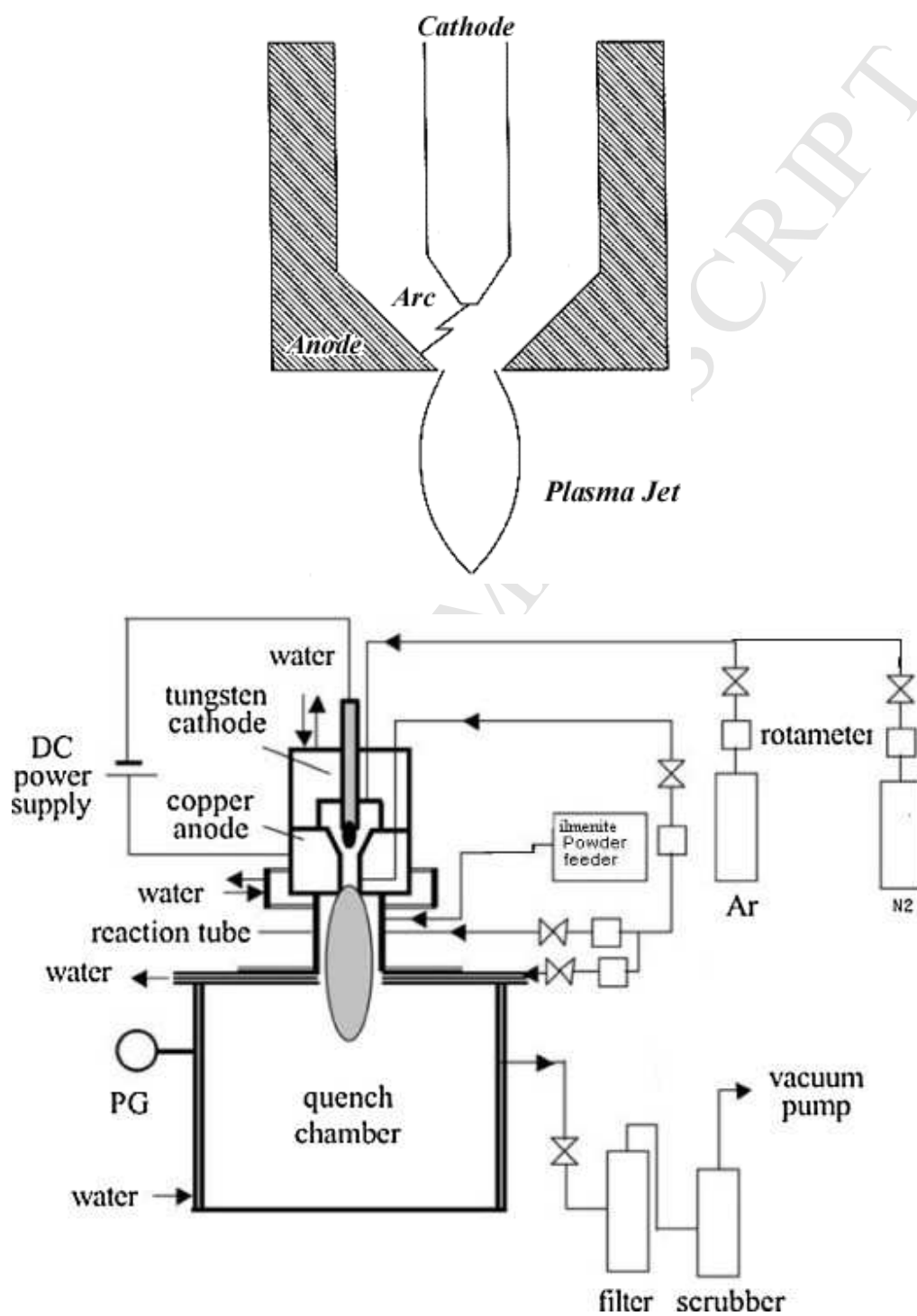
Fig. 8 Schematic diagram and example of non transferred arc reactor.
