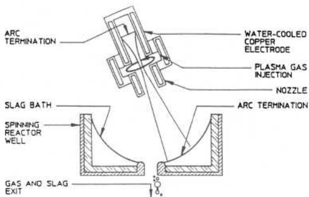
Fig. 16. Plasma technique for slag metallurgy.
