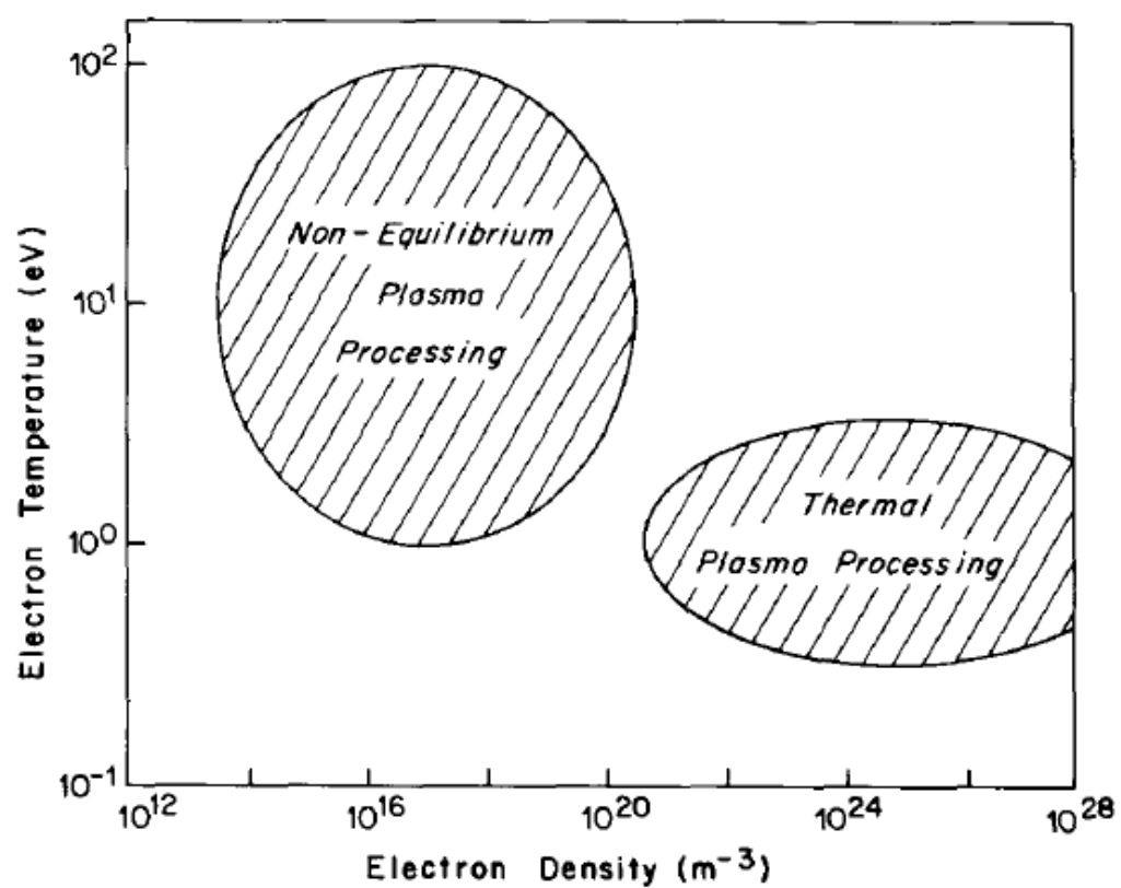
Fig. 2. Typical ranges of electron temperature range with electron density for non equilibrium and equilibrium plasma processing system.
