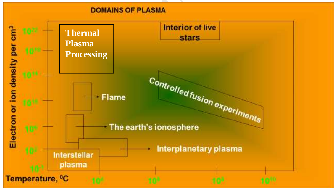
Fig. 1. Domains of plasma as the function of temperature and electron density.
