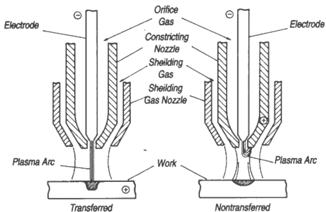
Fig. 7 Schematic diagram of transferred and non transferred arc reactors.
