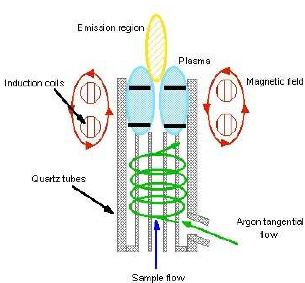
Fig. 12 Schematic diagram of RF inductively coupled discharge
