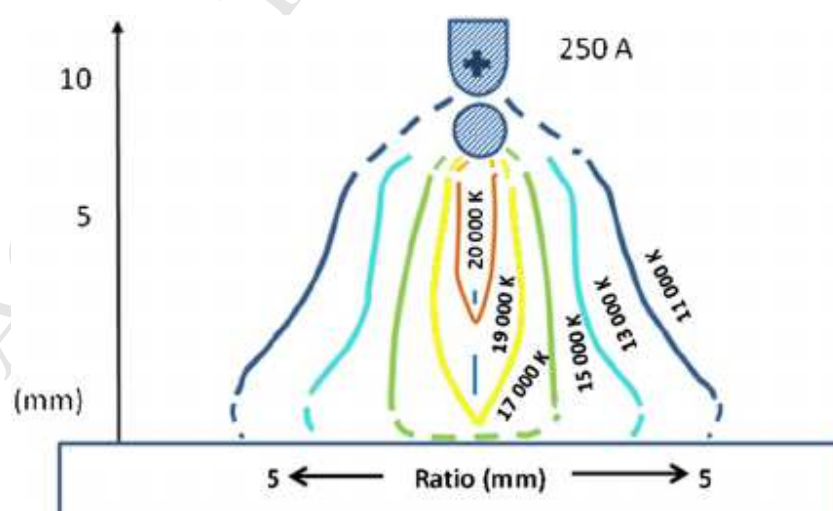
Fig. 6. Various zone of temperature distribution in arc thermal plasma .
