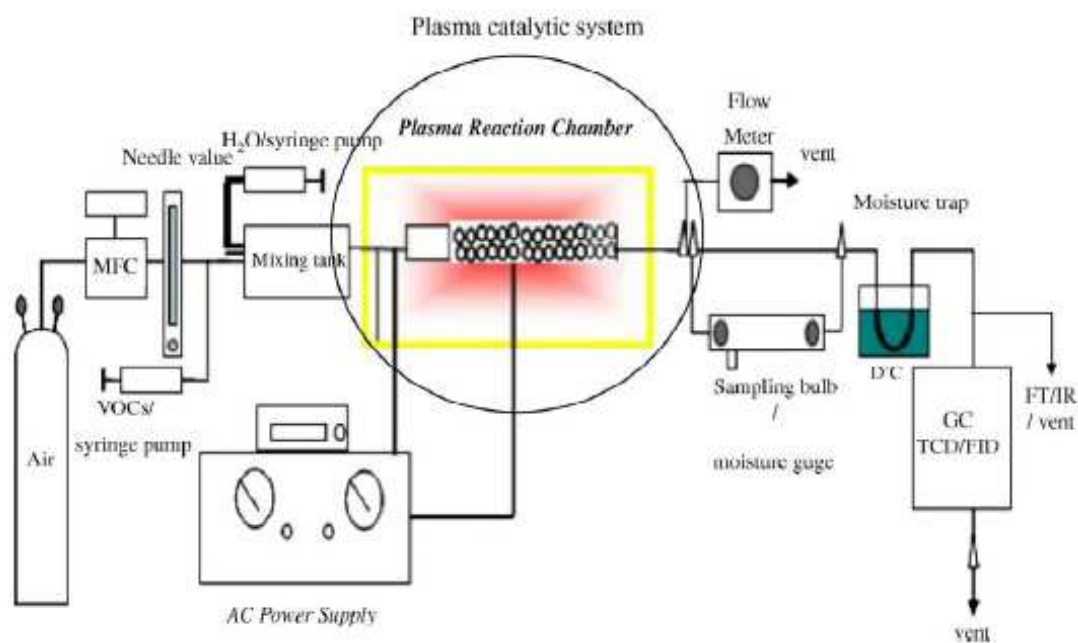
Figure 13 Schematic representation of discharge plasma reactor apparatus.
