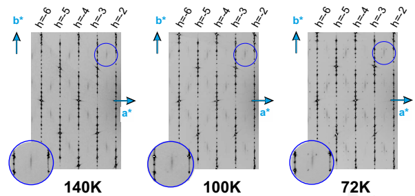
FIG. 1. Region of the (h0l)^* plane assembled from frames collected at T = 140 K, T = 100 K, T = 72 K. The diffuse scattering observed for the position \frac{\mathbf{a}^*}{2} weakened noticeably above T_{P1} while satellite reflections appear in irrational position.
