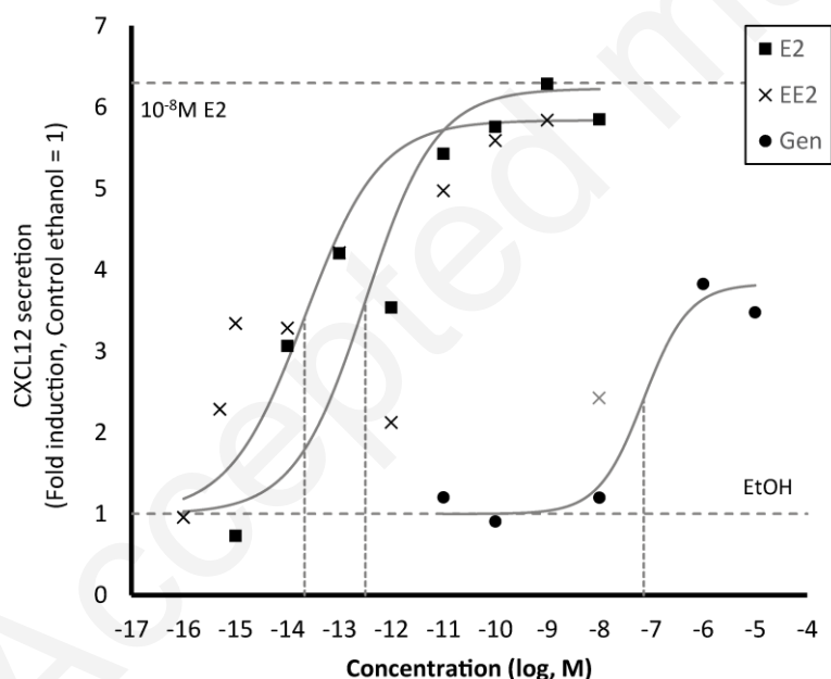
Fig. 1: CXCL12 secretion under classical estrogenic compounds stimulation in 96 well plate.
