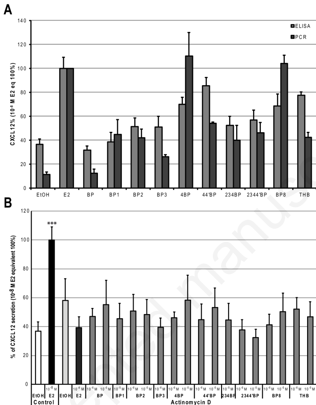
Fig. 5: A) Evolution of CXCL12 secretion and CXCL12 expression measured respectively by ELISA and qPCR after stimulation with E2 at 10^{-8} M and benzophenones at 10^{-6} M. B) CXCL-test performed on cells treated or not with control ethanol, E2 and effective doses of benzophenones with or without actinomycin D.
