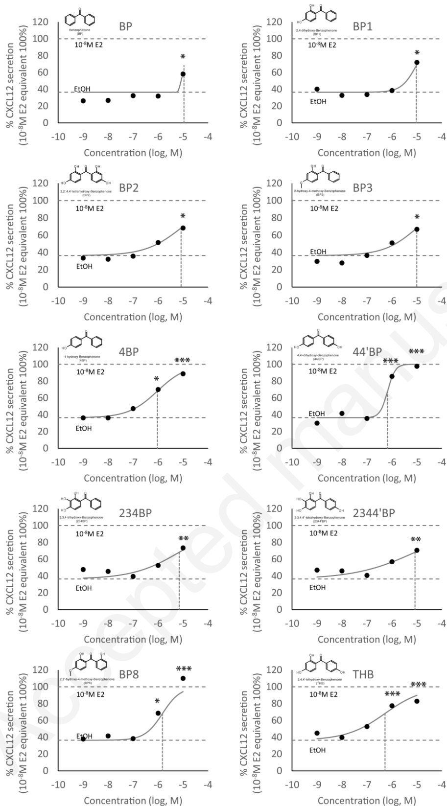
Fig. 4: Assessment of estrogenic properties of different doses of benzophenones (BP, BP1, BP2, BP3, 4BP, 44'BP, 234BP, 2344'BP, BP8 and THB) using CXCL-test.
