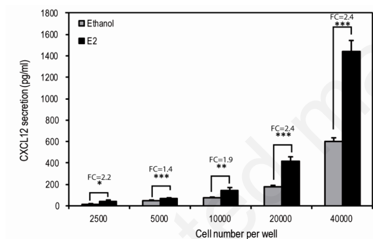
Fig. 2: CXCL12 secretion depending upon the cell number coated in the 96 well plate and without PBS/BSA intermediary dilution. (*P<0.05, **P<0.01, ***P<0.005)
