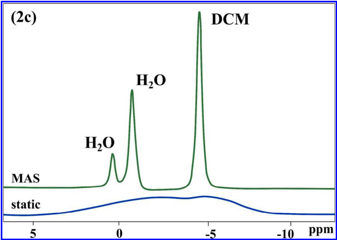
Figure 2. Static and MAS (9 kHz) spectra on THC515: (a) benzene (2.0 mol.kg -1 ); (b) mixture of benzene (2.0 mol.kg -1 )/cyclohexane (1.2 mol.kg -1 ); (c) dichloromethane (DCM) (2.5 mol.kg -1 )/water (2.3 mol.kg -1 ).
