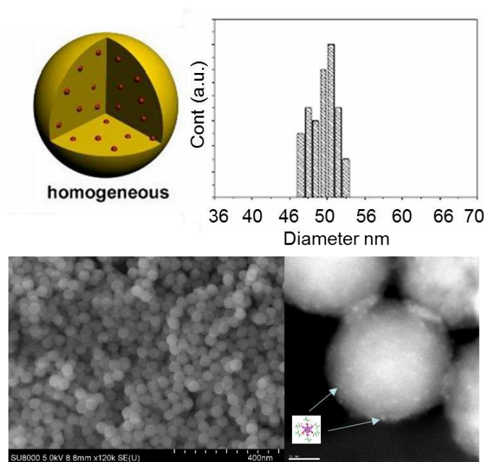
Fig. 2. Schematic homogeneous nanoparticle (top left). SEM (bottom left, bar is 400 nm) and HAADF-STEM (bottom right, bar is 10 nm) images of \text{Cs}_2\text{Mo}_6\text{I}_8(\text{C}_2\text{F}_5\text{COO})_6@/\text{SiO}_2 and histogram of the diameter (top right).
