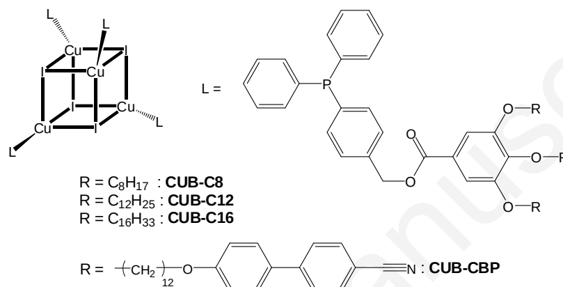
Figure 1. General representation of the functionalized [\text{Cu}_4\text{I}_4\text{L}_4] copper iodide clusters ( CUB ) with the corresponding \text{L} ligands with \text{Cn} ( n = 8, 12 and 16 ) for alkyl chains and CBP for cyanobiphenyl group.
