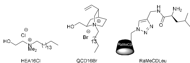
Figure 1. Structure of CDs and surfactants
