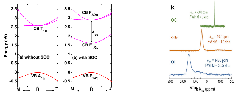
(a) Computed tight-binding diagram without SOC. (b) Corresponding band diagram with SOC. (c) ^{207}\text{Pb} MAS NMR spectrum obtained at 14T on \text{CH}_3\text{NH}_3\text{PbX}_3 .
