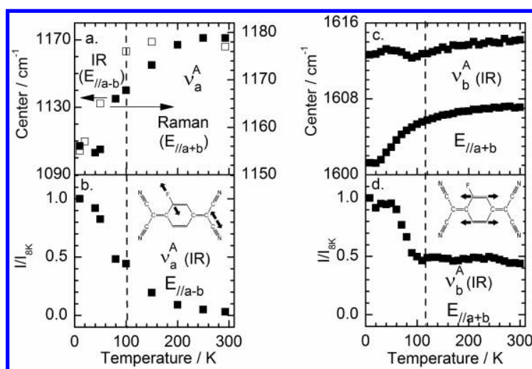
Figure 7: (a) Temperature evolution of the frequency of the TCNQF \nu_a^A band observed in the optical conductivity spectra (■) and in the Raman spectra (□); (b) temperature dependence of the intensity (normalized to 8 K value) of the TCNQF \nu_a^A band observed in the optical conductivity spectra; (c) temperature evolution of the frequencies of the two components of the TCNQF \nu_b^A band observed in the absorbance spectra; (d) temperature dependence of the intensity (normalized to 8 K value) of the TCNQF \nu_b^A doublet band observed in the absorbance spectra.
