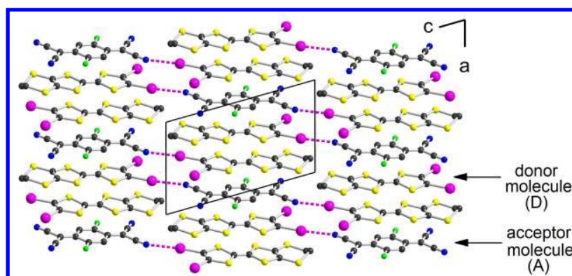
Figure 1: Projection view along b axis of the extended unit cell of (EDT-TTF-I 2 ) 2 TCNQF, showing the alternated ...ADDADDA... stacks. The pink dotted lines indicate the halogen bond interaction between iodine and nitrogen atoms. The single fluorine atom is disordered on two positions related by inversion center.
