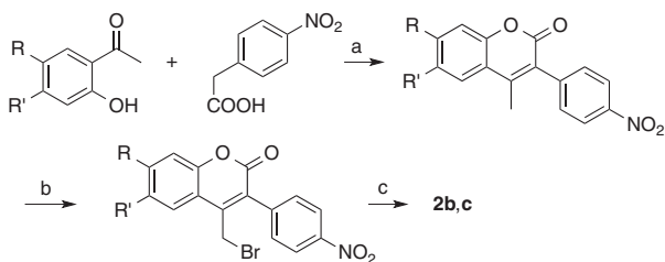
Scheme 1. Synthesis of 2b and 2c . a) Acetic anhydride, triethyl amine, 65 °C to RT, overnight, 51% yield. b) NBS, benzoyl peroxide, CCl 4 , 90 °C, 15 h, 40% yield. c) benzoic acid, K 2 CO 3 , KI, DMF, 50 °C, 6 h, 20% yield.
