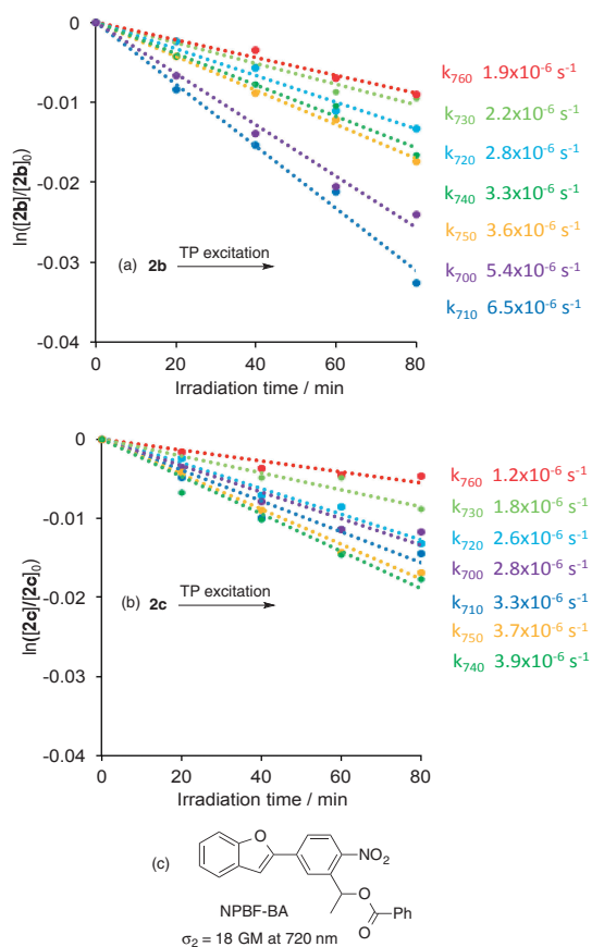
Figure 4. Time profile of the TP uncaging of (a) 2b and (b) 2c , \ln([\text{sub}]/[\text{sub}]_0) vs. irradiation time at wavelengths of 700, 710, 720, 730, 740, 750, and 760 nm at 700 mW. (c) TP reaction of NPBF-BA at 720 nm, \sigma_2 = 18 GM at 720 nm.
