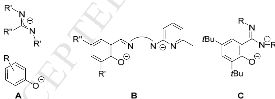
Scheme 1. Mixed ( A ) and hybrid ( B , C ) phenoxy-amidinate ligand systems used in the development of polymerization catalysts.
