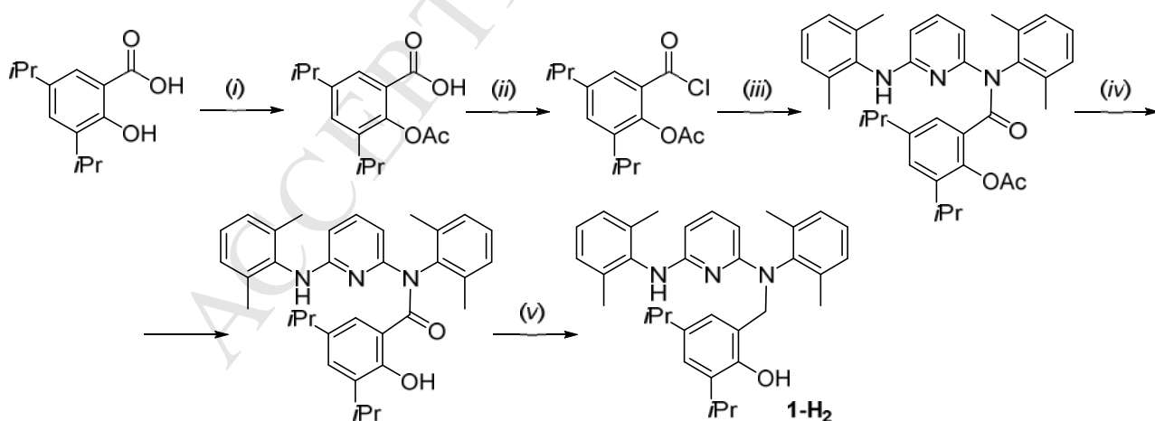
Scheme 2. Synthesis of the hybrid amidine-phenolate proligand [N^{Me_2}NN^{Me_2}C^{iPr_2}O]H_2 ( 1-H 2 ).
