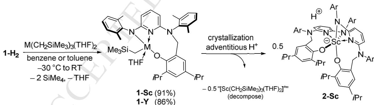
Scheme 3. Synthesis of complexes 1-Sc , 1-Y and isolation of 2-Sc .
