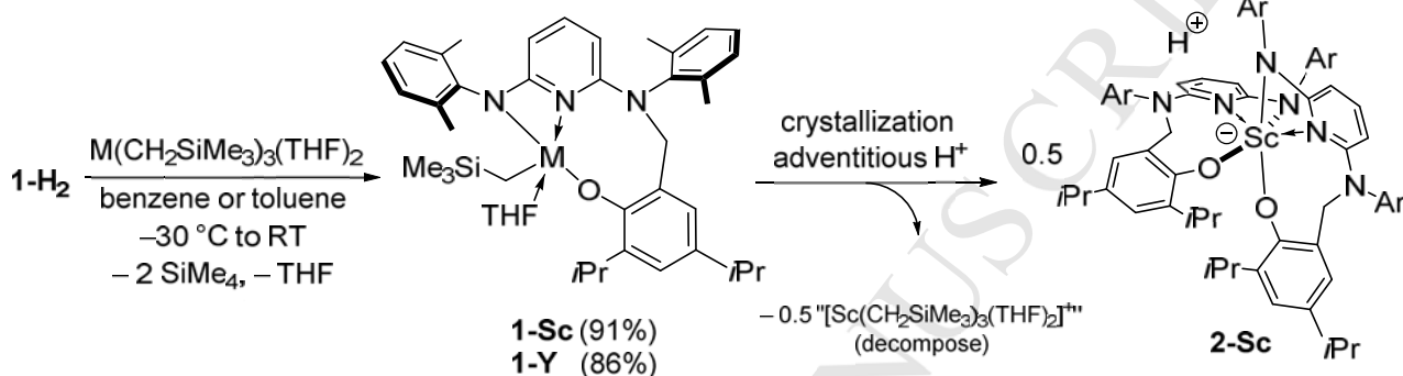
Scheme 2. Synthesis of complexes 1-Sc , 1-Y and isolation of 2-Sc .
