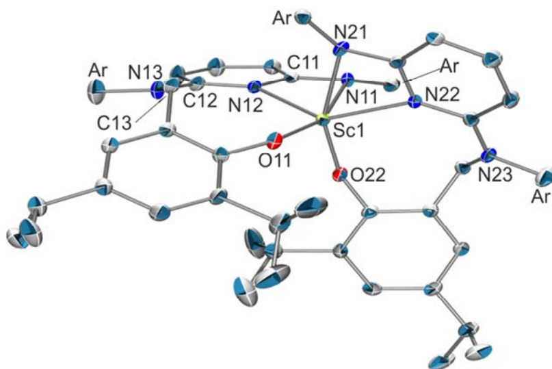
Figure 2. Molecular structure of 2-Sc (all hydrogen atoms and the four 2,6-dimethyl-phenyl groups (Ar) are omitted for clarity; thermal ellipsoids drawn at the 50% probability). Selected bond distances (Å) and angles (°): Sc(1)–N(11), 2.331(3); Sc(1)–N(12), 2.258(2); Sc(1)–O(11), 1.921(2); Sc(1)–N(12), 2.331(3); Sc(1)–N(22), 2.258(2); Sc(1)–O(22), 1.921(2); C(11)–N(11), 1.427(5); C(11)–N(12), 1.383(6); C(12)–N(12), 1.360(6); C(12)–N(13), 1.360(4); N(11)–Sc(1)–O(11), 158.50(10); N(12)–Sc(1)–N(21), 87.15(10); O(11)–Sc(1)–O(22), 99.24(15).
