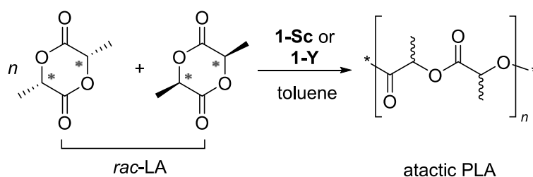
Scheme 3. Ring-opening polymerization of rac -LA.
