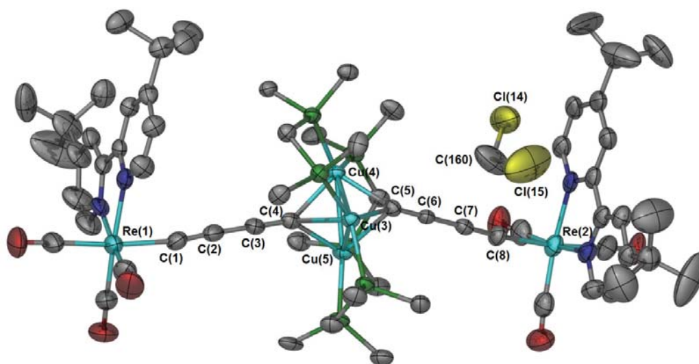
Fig. 5. A representation of the molecular structure of [\text{Cu}_3(\mu\text{-dppm})_3\{\mu_3\text{-C}\equiv\text{CC}\equiv\text{C}[\text{Re}(\text{CO})_3(\text{Bu}^{12}\text{-bpy})]\}_2]\text{PF}_6 [10] \text{PF}_6 showing the solvate \text{CH}_2\text{Cl}_2 molecule located between the \text{Cu}_3(\text{dppm})_3 cluster and the \text{Re}(\text{CO})_3(\text{Bu}^{12}\text{-bpy}) capping moiety. Ellipsoids have been drawn at the 50% probability level with remaining solvate molecules, the anion, hydrogen atoms and the phenyl carbons of the dppm ligands (except the ipso -carbons) omitted for clarity.
