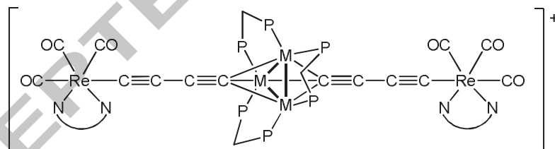
[M_3(dppm)_3\{C\equiv CC\equiv C[Re(CO)_3(NN)]_2\}]PF_6 M = Cu, Ag ; 10 M = Cu , NN = Bu^t_2-bpy
