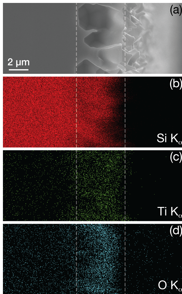
FIGURE 5. a) SEM cross section of a porous Si layer after ALD of \text{TiO}_2 ( N = 1400 cycles) and corresponding EDX mapping of the same area for b) Si \text{K}\alpha , c) Ti \text{K}\alpha and d) O \text{K}\alpha peaks.
