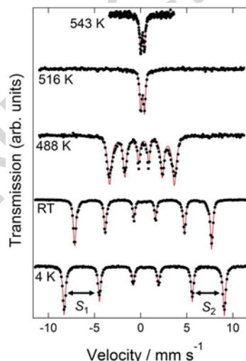
Figure 5. 57 Fe Mössbauer spectra of LiNbO 3 -type InFeO 3 at various temperatures. The dots represent the experimental data, and the solid red lines the total fits. S 1 and S 2 denote the relative shifts of the peaks.
