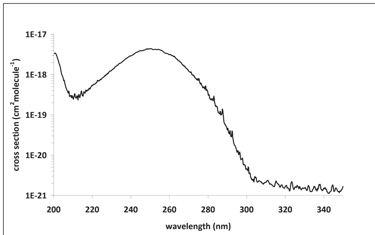
Figure 1: UV absorption spectrum of pyridine obtained in this work over the spectral range 200-350 nm at 353±1 K.
