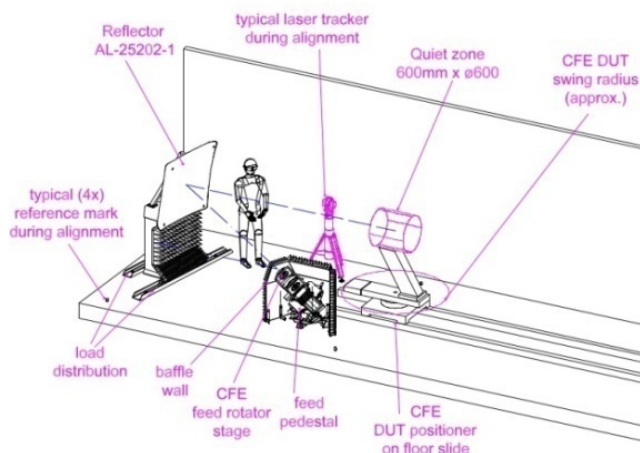
Figure 2. Overall view of the Compact Antenna Test Range.
