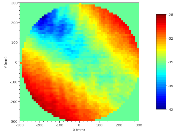
Figure 9. Horizontal field probe orientation: crosspolar magnitude results in dB limited to the QZ area
