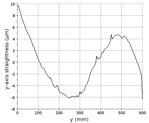
Figure 5. Mechanical probing procedure : y axis straightness results
