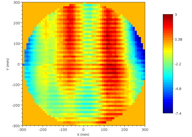
Figure 8. Horizontal field probe orientation: copolar phase results in degrees limited to the QZ area
