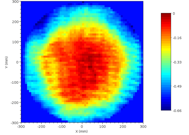
Figure 7. Horizontal field probe orientation: copolar magnitude in dB results limited to the QZ area.
