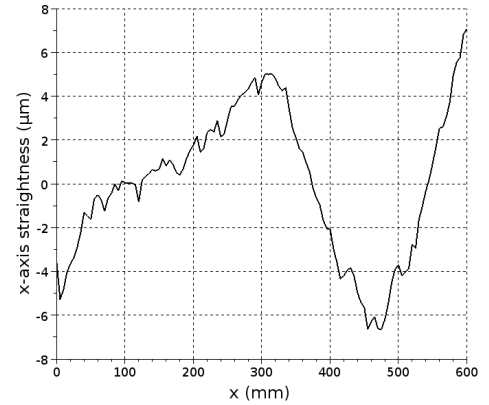
Figure 4. Mechanical probing procedure : x axis straightness results.
