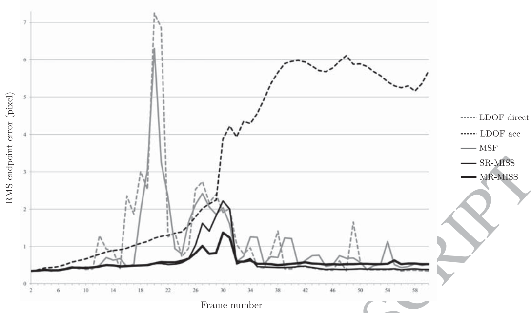
Figure 9: RMS endpoint errors for each pair \{I_{ref}, I_n\} along Flag sequence [25] with LDOF direct, LDOF acc, MSF [16, 17], SR-MISS [19] and our multi-reference frames strategy MR-MISS with \{I_1, I_{20}\} as reference frames.
