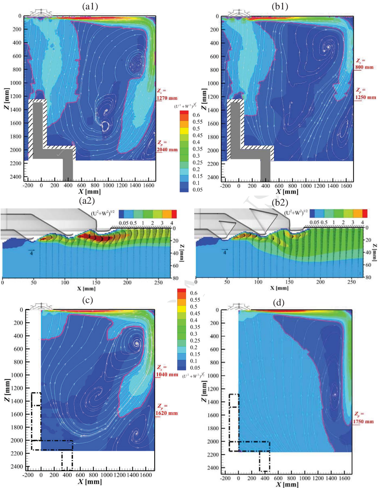
Fig. 5 Isocolors of velocity magnitude for Q_0=200 m 3 /h in the half middle cross section of the room,,: (a1) CD_CJ_HM, (b1) LD_CJ_HM, (c) CD_CJ, (d) CD_IJ - hatching zone around the manikin corresponds to the laser scattering, the magenta line represents 0.1 m/s isocontour; (a2, b2) Isocolors of velocity magnitude and vector profiles in the ceiling jet region for cases CD-CJ_HM and LD_CJ_HM
