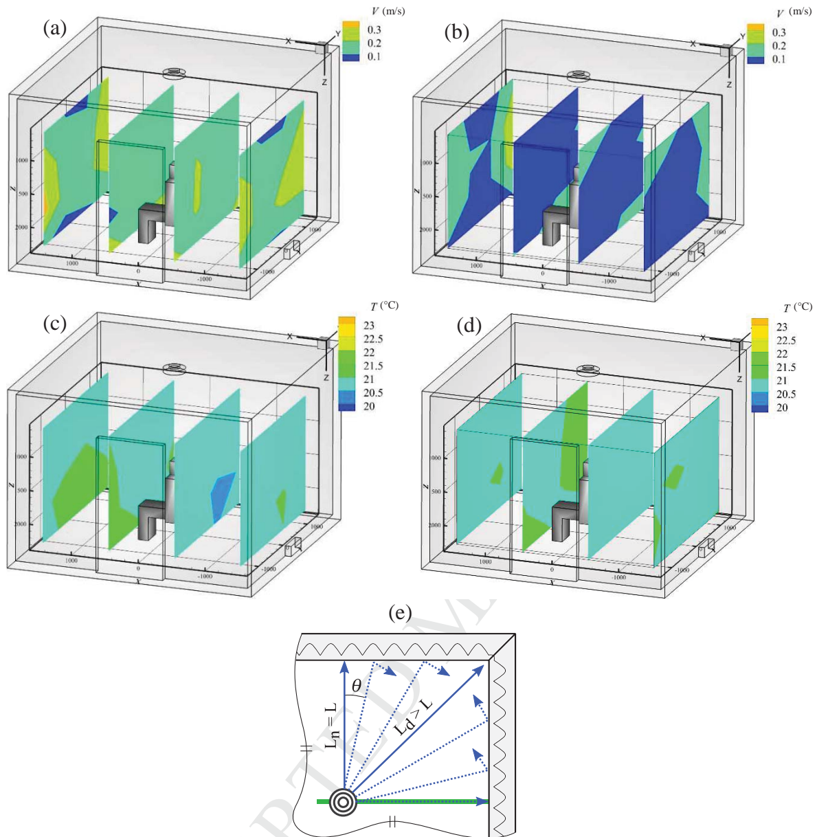
Fig. 11 Distributions of velocity magnitude (a, b), and air temperature (c, d) for Q_0 = 300 \text{m}^3/\text{h} , in CD_CJ_HM (left) and LD_CJ_HM (right). (e) Sketch of ceiling radial jet impingement on the wall and of confluence of downhill flows towards a corner – the green line symbolizes the laser plane in LS-PIV measurements
