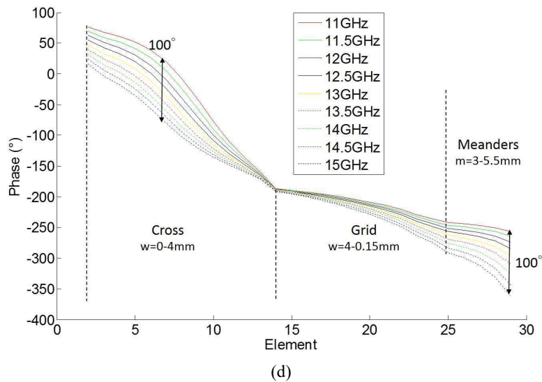
Fig. 7. Simulated performance of a phase-shifting cell with a “Meandered” grid a Metallic grid and unit cell with meanders of variable length m b Equivalent reactive effect of a simple grid and of a grid with meander for y-polarization c Complete phase range provided by the reflectarray cell d Phase variation over the complete cycle for different frequencies
