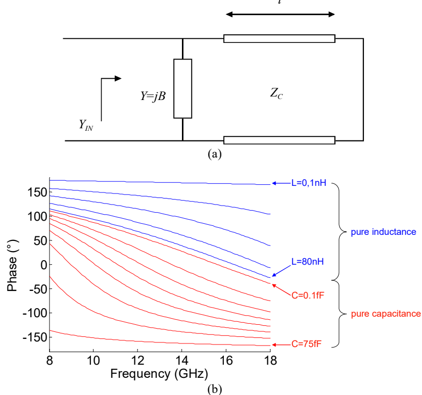
Fig. 3. Ideal performance of a phase-shifting cell a Equivalent circuit of a reflectarray cell composed of a pure reactive element above a ground plane b Ideal reflected phase versus frequency for different values of the pure capacitance C and the pure inductance L
