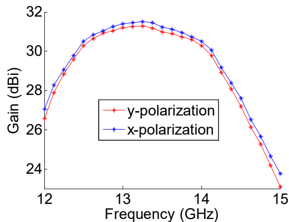
Fig. 12. Gain versus frequency in both polarizations
