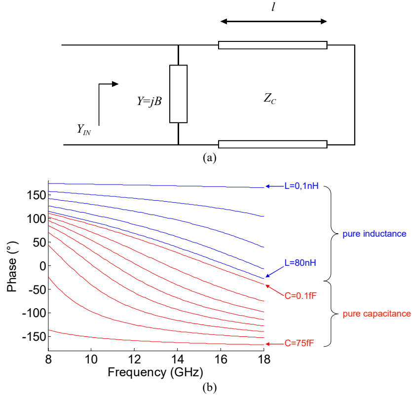
Fig. 3. Ideal performance of a phase-shifting cell
