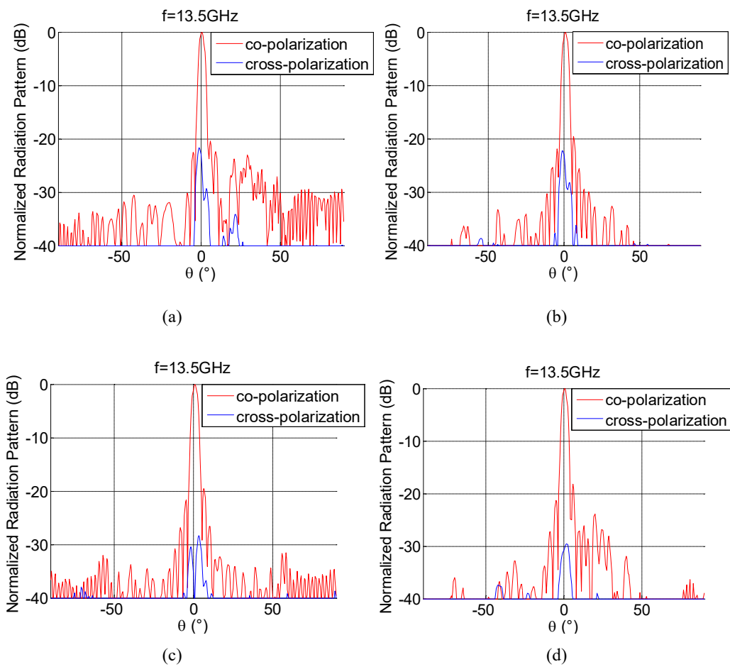
Fig. 10. Normalized radiation pattern measured at 13.5GHz a E plane when the electric field is y-polarized (vertical polarization) b H plane when the electric field is y-polarized (vertical polarization) c E plane when the electric field is x-polarized (horizontal polarization) d H plane when the electric field is x-polarized (horizontal polarization)
