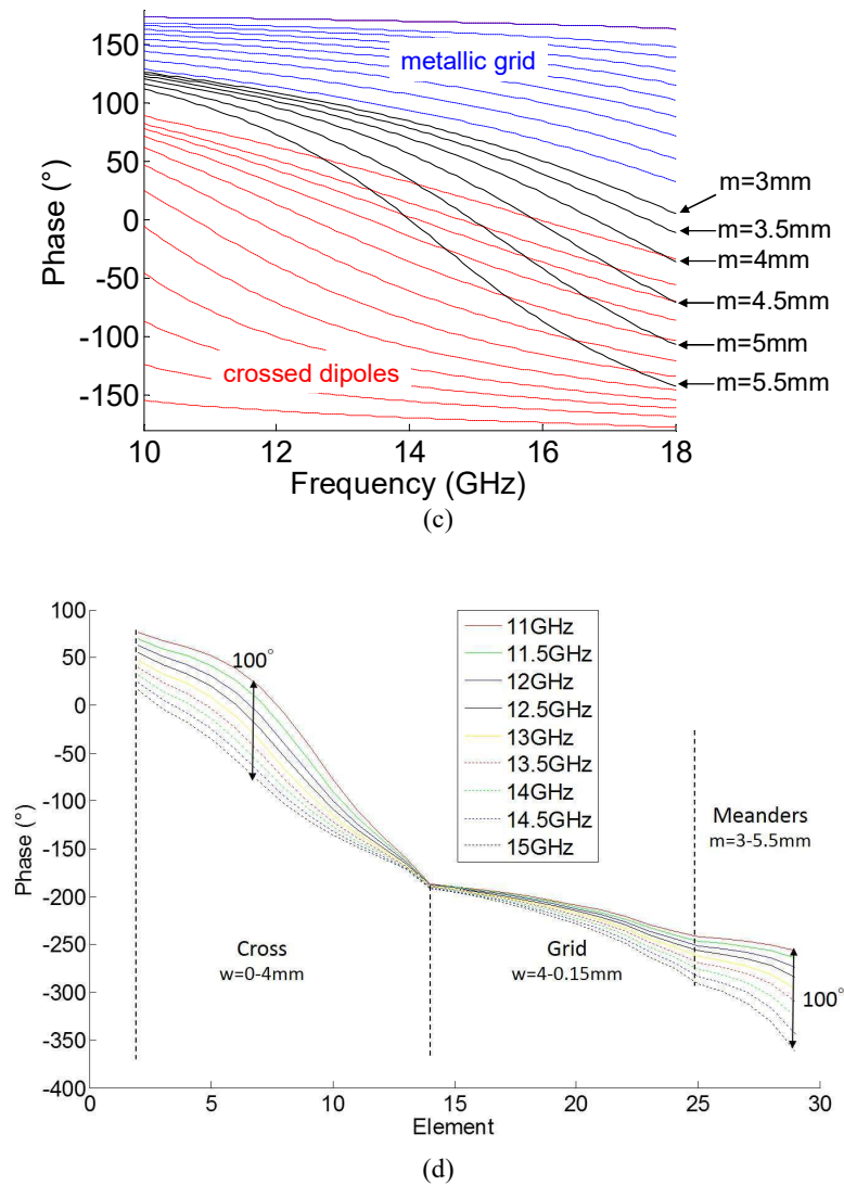
Fig. 7. Simulated performance of a phase-shifting cell with a "Meandered" grid
