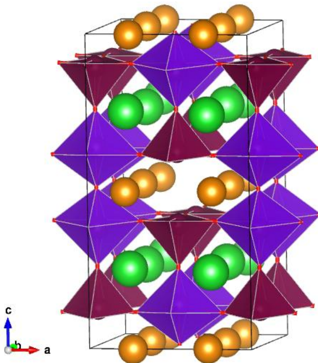
Figure 13. Crystal structure of NdBaMn 2 O 5.5 (S.G. Icmā ); Ba and Nd atoms are represented by green and gold spheres, respectively, Mn1 are in the pyramids and Mn2 in the octahedra, the different sites for the oxygen atoms are indicated.
