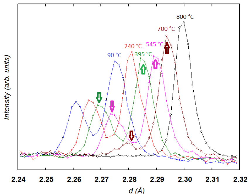
Figure 19. Selected region of the neutron diffraction patterns collected on heating the sample under wet 5% H 2 /He in the last cycle (indicated temperatures are average values). The arrows indicate conversion of NdBaMn 2 O 5.5 to NdBaMn 2 O 5.0 proceeding in the temperature range of 395-700 °C. The data set at 800 °C consists of the single NdBaMn 2 O 5 phase.
