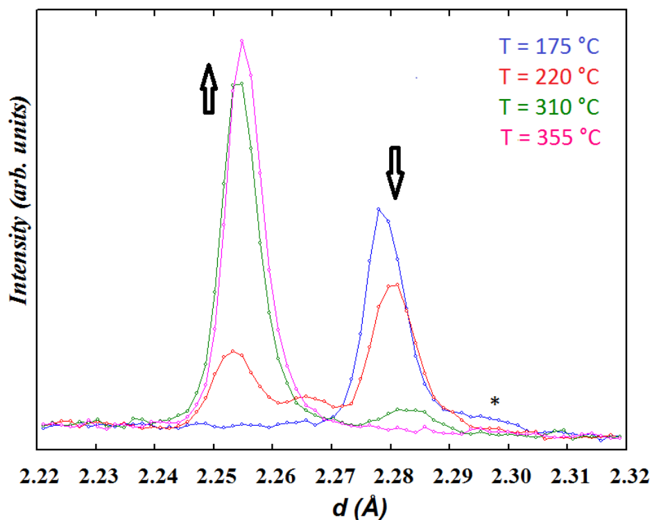
Figure. 8 Selected region of the neutron diffraction patterns collected every 15 minutes on heating \text{NdBaMn}_2\text{O}_{5+\delta} under flowing. The additional peak (*) that appeared on cooling under hydrogen in cycle 1 disappeared as the oxidation is progressing.
