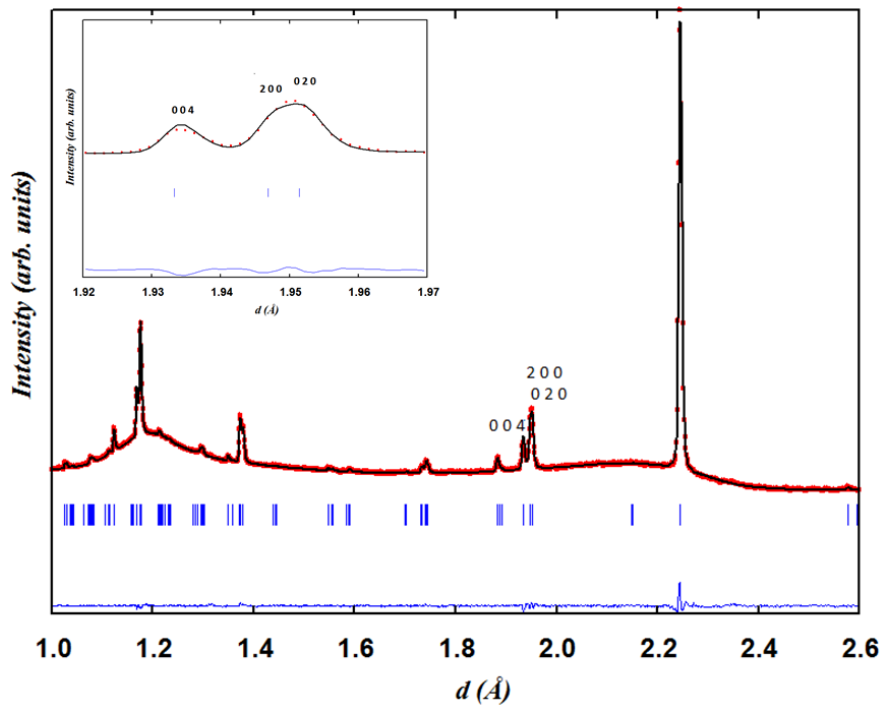
Figure 11. Neutron powder diffraction profile (backscattering bank) of \text{NdBaMn}_2\text{O}_{6-\delta} (S.G. Pmmm ) collected at 65 °C for 2 h after a heating/cooling cycle under flowing air; the orthorhombic distortion is evidenced by the (200/020) doublet highlighted in the inset.
