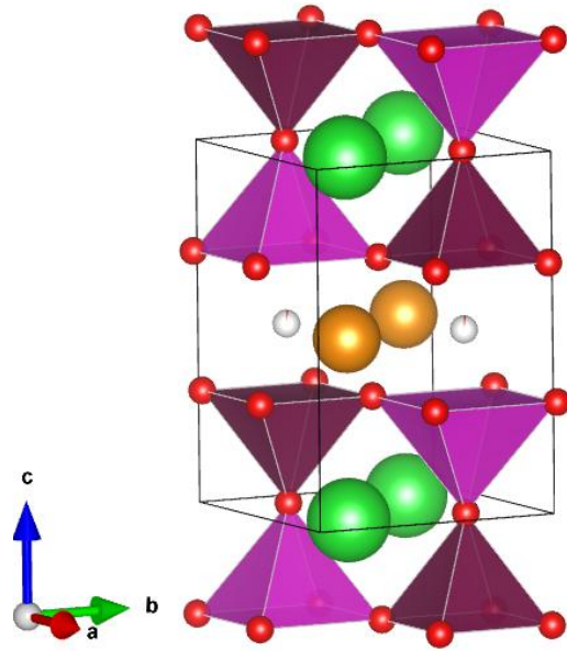
Figure 2. Schematic crystal structure of NdBaMn 2 O 5 (S.G. P4/nmm ) with (burgundy) Mn 3+ O 5 and (purple) Mn 2+ O 6 forming double pyramidal layers containing (green) Ba 2+ cations and interleaved with (gold) Nd 3+ layers.
