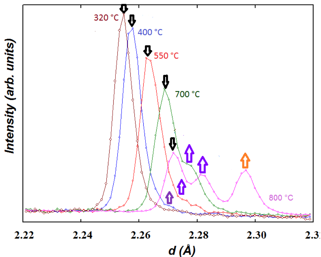
Figure 12. Selected region of the neutron diffraction patterns collected on heating \text{NdBaMn}_2\text{O}_{6-\delta} under 5% \text{H}_2/\text{He} (cycle 3), indicated temperatures are average values). The arrows indicate decrease or increase of the different coexisting phases; black: “ \text{O}_6 ”, purple: “ \text{O}_{5.5} ” and yellow: “ \text{O}_{5.0} ”.
