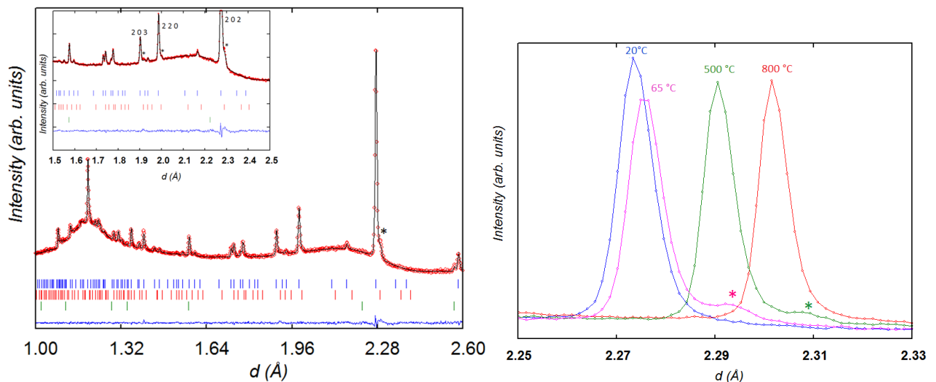
Figure 7. Neutron powder diffraction profile at 65 °C after cycle 1 of the sample consisting of \text{NdBaMn}_2\text{O}_5 (upper markers), the new phase (middle markers) and MnO (lower markers) with insight highlighting a few peaks (*) of the new phase. (Right) evolution of the (202) peak of \text{NdBaMn}_2\text{O}_5 and main peak (*) originating from the new phase on cooling.
