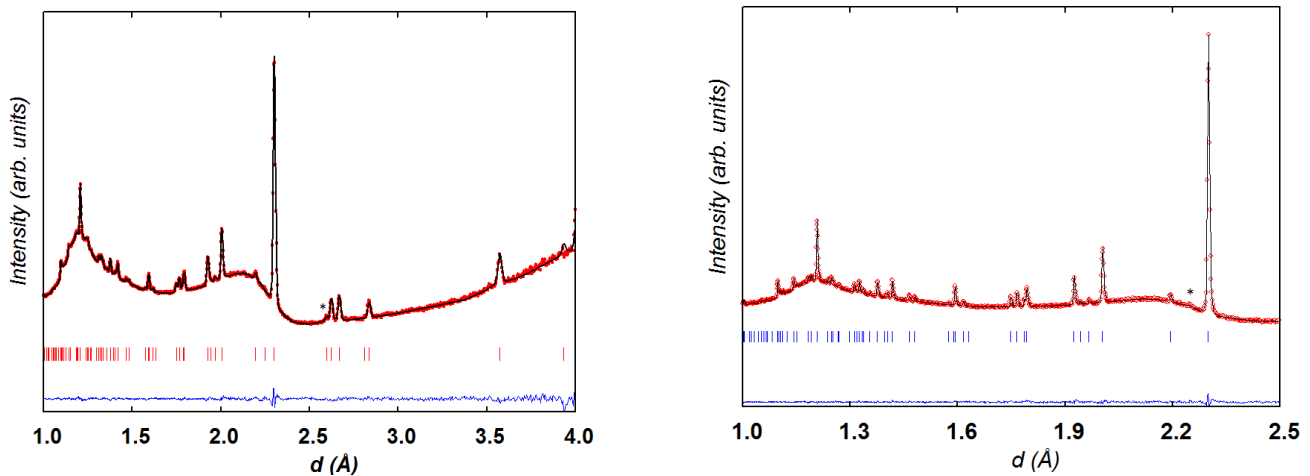
Figure 5. Neutron powder diffraction profiles for the sample NdBaMn 2 O 5 800 °C under 5% H 2 /He; S.G. P4/nmm , \chi^2 \sim 2.23 , (left) fitted 2\theta \sim 90^\circ bank data, (right) fitted backscattering profile. The asterisks relate to peaks from MnO impurity.
