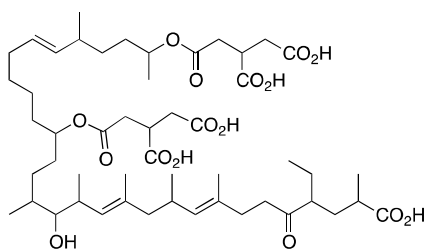
24: Actinoplanic acid B
