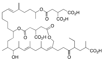
23: Actinoplanic acid A
