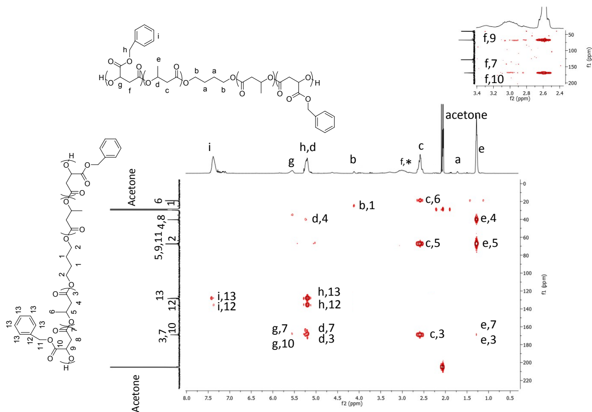
Figure S7. ^1\text{H} - ^{13}\text{C} HMBC NMR (400 MHz, acetone- d_6 , 23 °C) spectrum of HO-PMLA Be 2200 - b -PHB 4900 - b -PMLA Be 2200 -OH synthesized by ROP of MLA Be from Nd(OTf) 3 /HO-PHB 4900 -OH (Table 1, entry 5).
