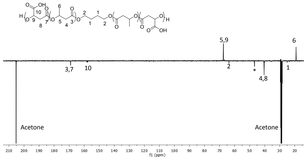
Figure S14. ^{13}\text{C}\{^1\text{H}\} J-MOD NMR (100 MHz, acetone- d_6 /TFA 98:02, v/v, 23 °C) spectrum of the HO-PMLA 1100 - b -PHB 4600 - b -PMLA 1100 -OH sample obtained upon hydrogenolysis of the HO-PMLA Be 2200 - b -PHB 4900 - b -PMLA Be 2200 -OH (Table 1, entry 5) (* marker stands for unidentified impurities).
