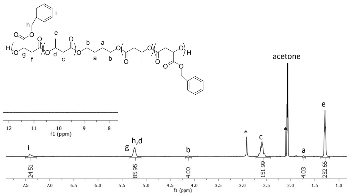
Figure S4. 1 H NMR (400 MHz, acetone- d 6 , 23 °C) spectrum of HO-PMLA Be 500 - b -PHB 6500 - b -PMLA Be 500 -OH sample synthesized by ROP of MLA Be from Nd(OTf) 3 /HO-PHB 6700 -OH (Table 1, entry 2) (* marker stands for residual water and acetone).
