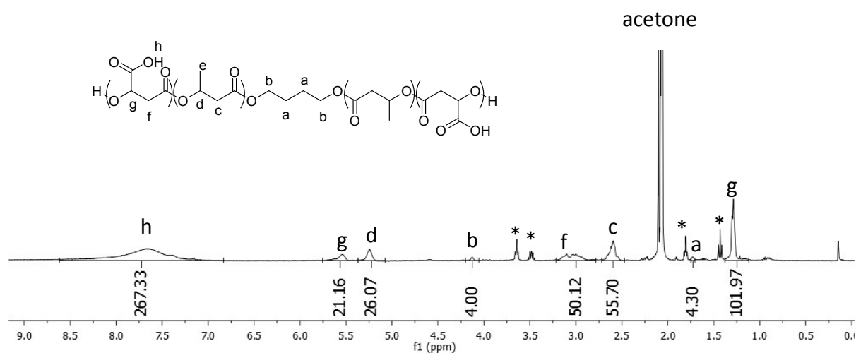
Figure S13. ^1\text{H} NMR (400 MHz, acetone- d_6 /TFA (98:02, v/v), 23 °C) spectrum of HO-PMLA- b -PHB- b -PMLA-OH obtained upon hydrogenolysis of HO-PMLA Be 4100 - b -PHB 2500 - b -PMLA Be 4100 -OH (Table 1, entry 6) (* marker stands for unidentified impurities).
