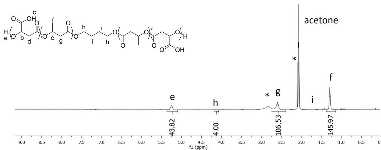
Figure S10. ^1\text{H} NMR (400 MHz, acetone- d_6 , 23 °C) spectrum of HO-PMLA 1100 - b -PHB 4600 - b -PMLA 1100 -OH obtained upon hydrogenolysis of HO-PMLA Be 2200 - b -PHB 4900 - b -PMLA Be 2200 -OH (Table 1, entry 5) (* marker stands for residual water and acetone). The signals of the PMLA block do not suitably integrate as the result of the partial solubility of this block in acetone.
