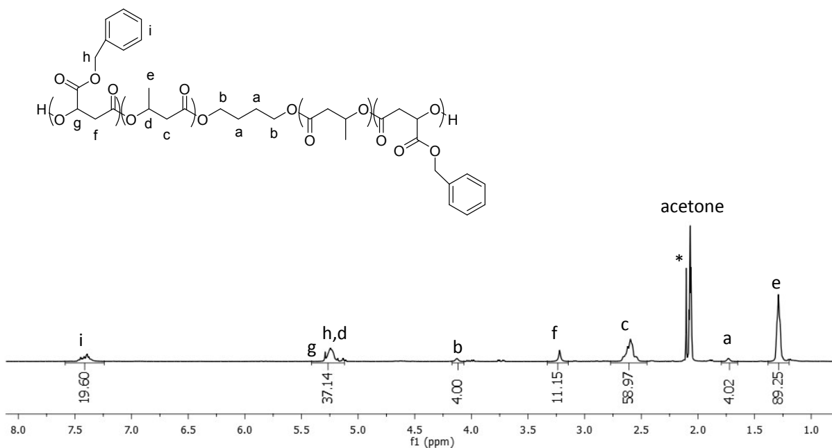
Figure S3. 1 H NMR (400 MHz, acetone- d 6 , 23 °C) spectrum of a HO-PMLA Be 400 - b -PHB 2500 - b -PMLA Be 400 -OH sample synthesized by ROP of MLA Be from Nd(OTf) 3 /HO-PHB 2700 -OH (Table 1, entry 1) (* marker stands for residual acetone).
