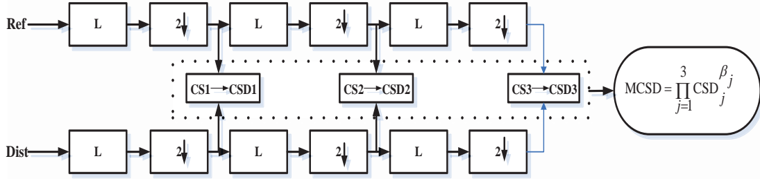
Fig.1. Structure diagram of the MCS D. Ref indicates a reference image and Dist indicates the corresponding distorted one, L: low-pass filtering; 2\downarrow : down sampling by 2; CS1, CS2 and CS3 mean contrast similarity map1, contrast similarity map2 and contrast similarity map3, respectively; CSD1, CSD2 and CSD3 mean the standard deviation of CS1, CS2 and CS3, respectively. The general idea of the MCS D is to decompose the reference and the distorted images into three scales, then calculate their contrast similarity deviation for each scale, and get the final note via a pooling of the CSD values on the three scales.
