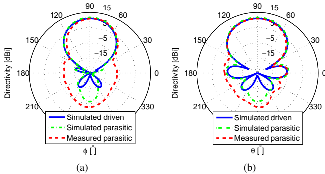
Fig. 5. Proposed array simulated and measured 2D total directivity radiation pattern. (a) Horizontal plane and (b) vertical plane.
