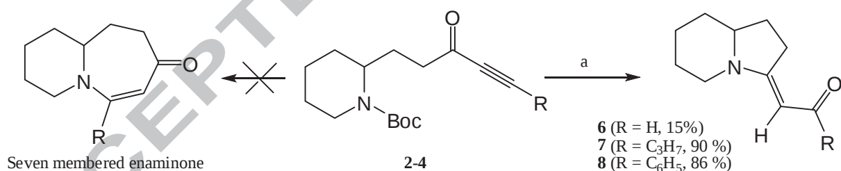
Scheme 2. Synthesis of amide vinylogues 6-8 . Reagents and conditions: (a) CH 3 SO 3 H (5 equiv), CH 2 Cl 2 /CH 3 OH, RT, 4 h then Na 2 CO 3 , 12 h.
