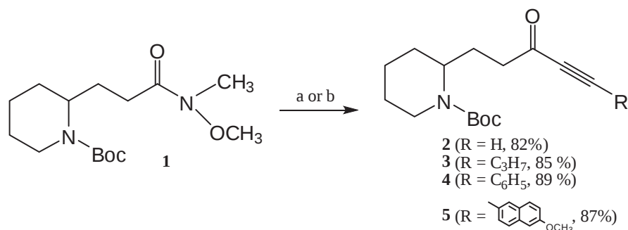
Scheme 1. Synthesis of starting materials 2 to 5 . Reagents and conditions: (a) H-C≡CMgBr, THF, 0 °C; (b) R-C≡CH, n BuLi, THF, -50 °C.
