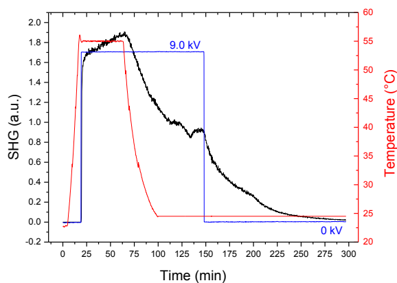
Fig. 3. In situ corona-wire poling dynamic of a PMMA film containing complex 2 , as host/guest system.
