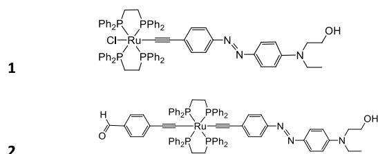
Scheme 1. Formulas of the two investigated complexes.
