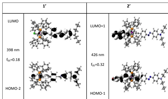
Fig. 2. Main molecular orbitals involved in the two lowest lying electronic transitions having sizeable oscillator strength ( f_{01} ) for compounds 1' and 2' . Corresponding wavelengths are also given. Both geometries and properties have been computed in the presence of solvent (DCM). The weight on the Ru atom amounts to 17 and 19% respectively in the HOMO and HOMO-2 of compound 1' and to 15 and 38% in the HOMO and HOMO-1 of compound 2' . C and H are depicted in grey, N, Cl, O, P and Ru are depicted in blue, green, red, orange and fuchsia, respectively.
