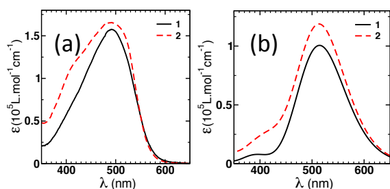
Fig. 1. UV-vis absorption spectra of compounds 1 and 2 in DCM (a) experimental spectra and (b) calculated spectra for a HWHM=2000 \text{cm}^{-1} .
