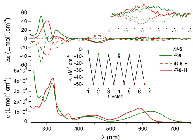
Figure 4. Top: ECD spectra (ca. 10^{-5} M) of M -6-H, P -6-H ( \text{CH}_3\text{CN} + \text{HBF}_4 ) and M -6, P -6 ( \text{CH}_3\text{CN} + \text{Et}_3\text{N} ). Bottom: absorption spectra of rac -6-H (red) and rac -6 (green) in \text{CH}_3\text{CN} , added for comparison. Insert: reversibility of pH-switching monitored at 300 nm for M -6/6-H.
