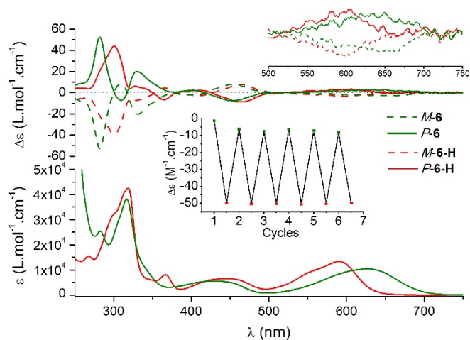
Figure 4. Top: ECD spectra (ca. 10^{-5} M) of M - 6-H , P - 6-H ( \text{CH}_3\text{CN} + \text{HBF}_4 ) and M - 6 , P - 6 ( \text{CH}_3\text{CN} + \text{Et}_3\text{N} ). Bottom: absorption spectra of rac - 6-H (red) and rac - 6 (green) in \text{CH}_3\text{CN} , added for comparison. Insert: reversibility of pH-switching monitored at 300 nm for M - 6/6-H .
