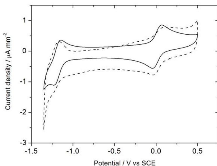
Figure 1. Cyclic voltammograms on a 3 mm diameter glassy carbon electrode in water + 0.1 mol L -1 Na 2 SO 4 + 0.1 mol L -1 HDTAB of 1.9 \times 10^{-3} mol L -1 of [Co(bpy(CH 2 OH) 2 ) 2 ] 2+ prepared from 2 (----) and 4 (—) eq. of [2,2'-bipyridine]-4,4'-diyldimethanol 8 . Scan rate 0.02 V s -1 .
