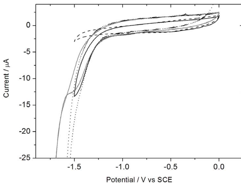
Figure 2. Cyclic voltammograms in 0.1 mol L -1 Na 2 SO 4 + 0.1 mol L -1 HDTAB without (----) and with 4 \times 10^{-3} mol L -1 alachlor (—), 4 \times 10^{-3} mol L -1 metazachlor (—), 4 \times 10^{-3} mol L -1 metolachlor (.....) on a 3 mm diameter glassy carbon electrode. Scan rate 0.02 V s -1 .
