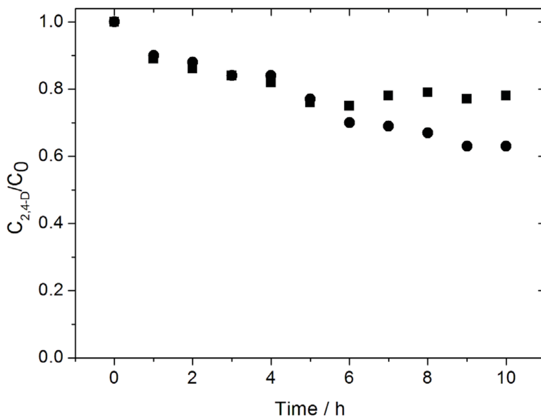
Figure 5. Exhaustive electrolysis. Evolution of the normalized concentration C_{2,4-D}/C_0 vs electrolysis time for the cathodic reduction of 2,4-D ( 4.5 \times 10^{-4} mol L -1 ) performed with [\text{Co}(\text{bpy}(\text{CH}_2\text{OH})_2)_2]^{2+} ( 2.3 \times 10^{-4} mol L -1 (■); 1.8 \times 10^{-4} mol L -1 (●)) in 0.1 mol L -1 Na 2 SO 4 (pH=7.2, 1 mL min -1 ).
