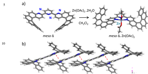
Scheme 2. a) Coordination of achiral ligand meso -1 to Zn 2+ , generating meso -1·Zn(OAc) 2 and their respective X-ray crystal structures. b) X-ray structure and supramolecular arrangement of ( P,P )-1 along the x axis in the solid state.
