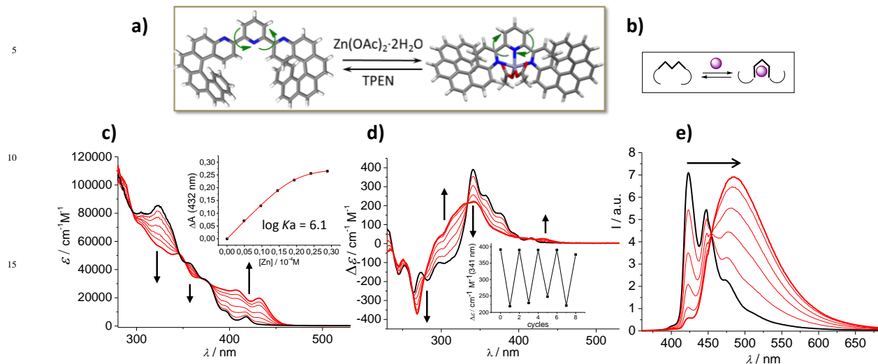
Figure 2. a) Reversible Zn(II) complexation-decomplexation process of ( P,P )- 1 using Zn(OAc) 2 and TPEN as the chemical stimuli. b) Schematic modification of the geometry. c) Evolution of the UV-vis spectrum of ( P*,P* )- 1 # ( 3 \times 10^{-5} M, CH 2 Cl 2 , rt) upon addition of Zn(OAc) 2 ·2H 2 O aliquots (0.2 equiv. until saturation at 1.0-1.2 equiv.). Inset: Absorption at 432 nm and fitting with a 1:1 binding model. d) Evolution of the ECD spectrum of ( P,P )- 1 . Inset: Reversible ECD 341nm switching process. e) Evolution of the fluorescence of ( P,P )- 1 ( \lambda_{\text{ex}} = 350 nm, 2.2 \times 10^{-5} M, CH 2 Cl 2 , r.t.).
