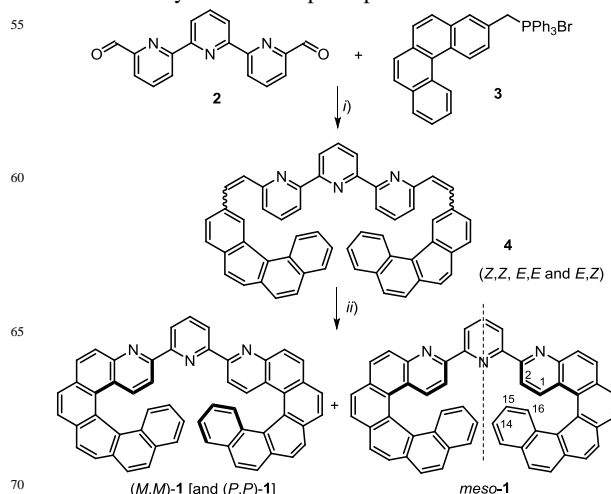
Scheme 1. Synthesis of bis-helicenic terpyridine 1 . i ) n -BuLi, THF, r.t., 5 h, 82%; ii ) hv, cat. I 2 , toluene/THF, r.t., 7 h, 45%.
