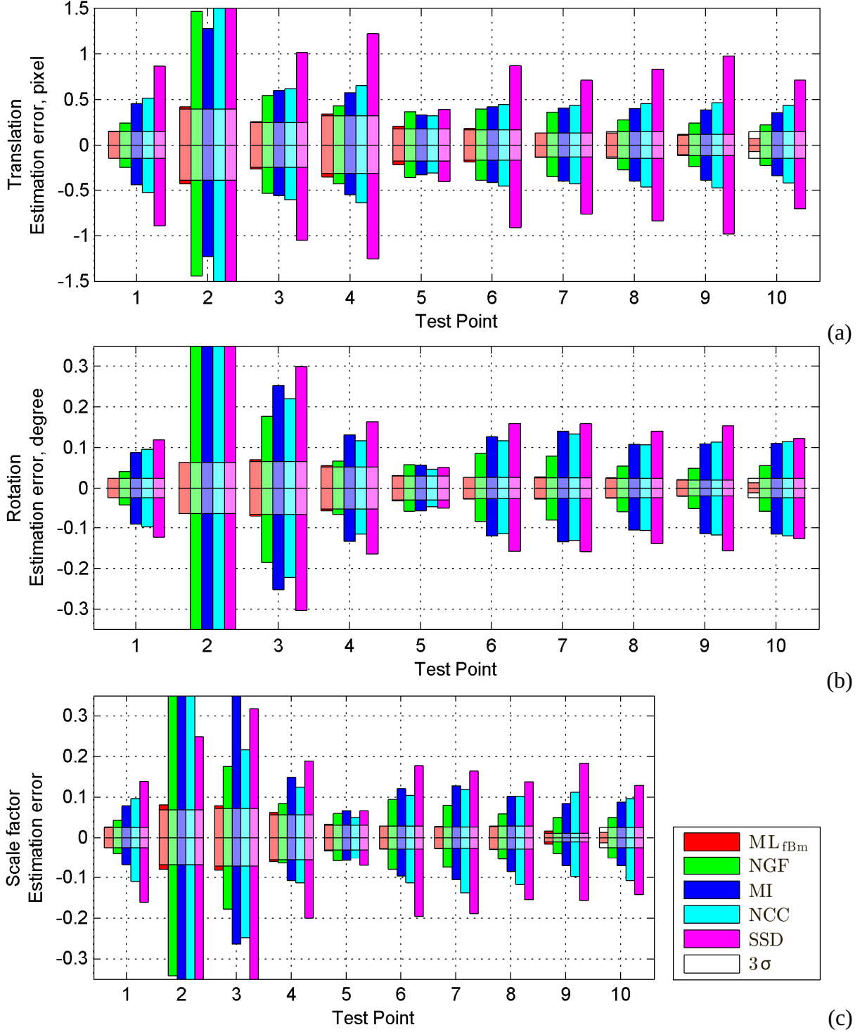
Fig. 2. Characteristics of RST parameters estimation errors for horizontal translation (a), rotation angle (b) and scaling factor (c) obtained by the five algorithms retained in the comparative study for all TPs #1-10
