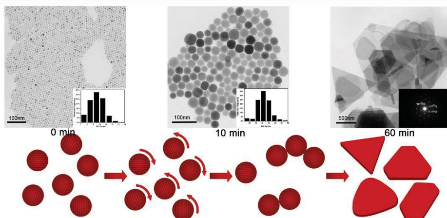
TEM images of the copper selenides nanoparticles and nanoplates synthesized at 180°C for 0 min, 10 min, 60 min. And the growth mechanism of the copper selenide nanoplates via the “oriented attachment”.
