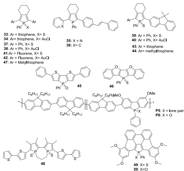
Fig. 7: Phosphole derivatives as emitters in OLED and WOLED
