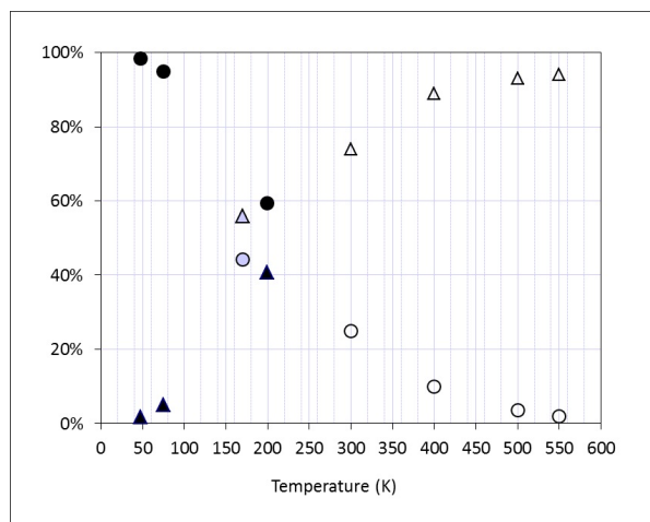
Figure 4: (●, ▲) Black full circles and triangles correspond to the observed \text{POCl}_3^- and \text{POCl}_2^- signal proportions (%) for the different temperatures 47.7, 74.5 and 199.5K. (○, △) Gray circles and triangles correspond to the \text{POCl}_3^- and \text{POCl}_2^- signal proportions respectively at 169.7K for which the density is lower, i.e. 0.572 \times 10^{16} molecule. \text{cm}^{-3} . (○, △) Open circles and triangles are the \text{POCl}_3^- and \text{POCl}_2^- branching ratios from (11).
