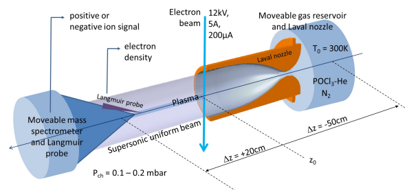
Figure 1: Supersonic cold uniform beam in the CRESU apparatus at Rennes.
