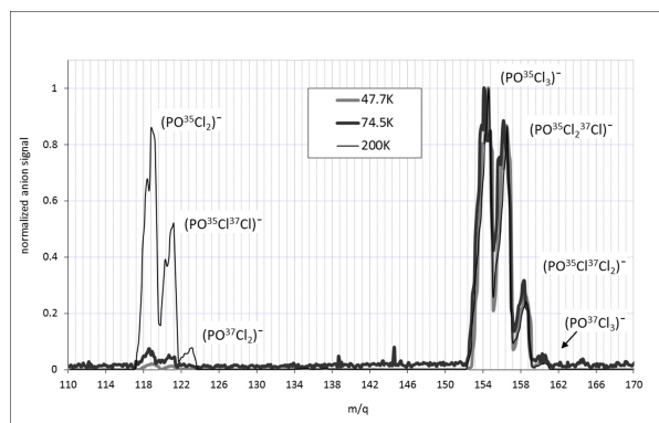
Figure 2: Normalized negative mass spectra for three different temperatures: 47.7, 74.5 and 199.5K. The typical density is about n_{tot} = 10^{16} molecules \text{cm}^{-3} (see Table 1 for details) and the distance between the mass spectrometer and the electron beam is 9 cm.
