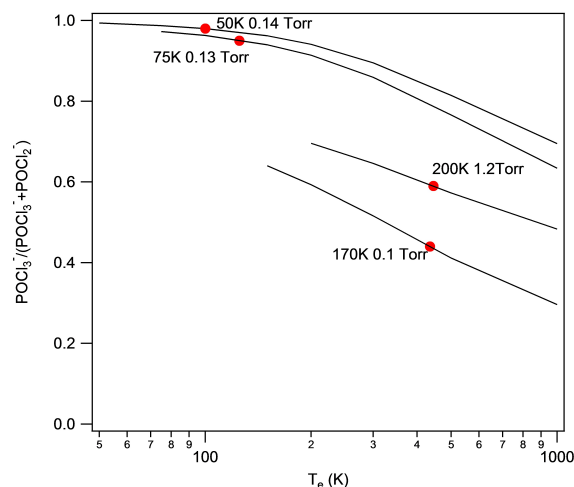
Figure 5: Non-dissociative branching fraction of attachment to \text{POCl}_3 (solid lines) from the kinetic model at the indicated densities and gas temperatures as a function of electron temperature. Full circles (●) are CRESU experimentally measured branching fractions at ill-defined electron temperatures and are plotted at the T_e where agreement with the modeling is best.
