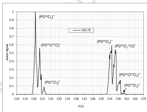
Figure 3: Normalized negative mass spectra for a molecular beam corresponding to a temperature T=169.7\text{K} and a density n_{tot} = 0.572 \times 10^{16} molecules/ \text{cm}^3 .
