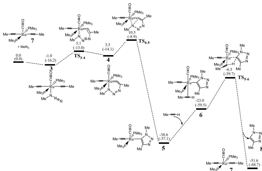
Fig. 9 DFT free energy profile (in kcal/mol) for the proposed mechanism of the formation of 1,4-triazole catalyzed by a Ru complex lacking cyclopentadienyl ligand. Reproduced with permission from ref. 29. Copyright 2012, American Chemical Society.
