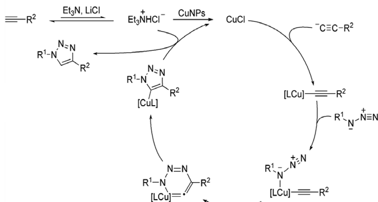
Figure 6. Reaction mechanism proposed for the CuNPs-catalyzed 1,3-dipolar cycloaddition of terminal alkynes and azides. Reproduced with permission from ref. 80. Copyright 2010, WILEY-VCH.
