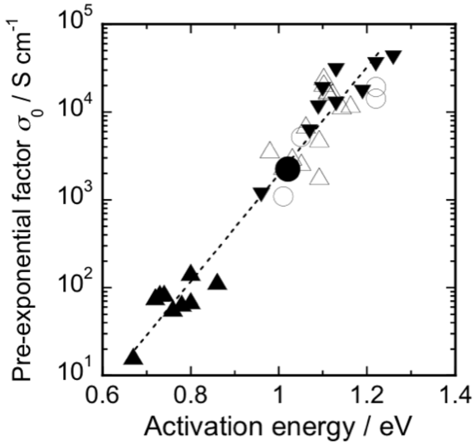
Figure 9. Relationship between the \Delta E and \log \sigma_0 for YSZ measured at various temperatures and compositions (varied the amount of Y_2O_3 ); ●: the FEM calculation result, \Delta : ref[43], \blacktriangle : ref [42] (High temperature), \circ : ref[41], \blacktriangledown : ref[42] (Low temperature).
