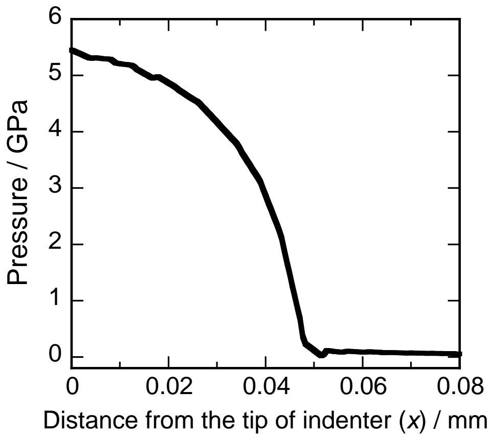
Figure 5. (a) 2D view of the pressure at Gauss point calculated by the FEM ( P = 25 N), and (b) the relationship between the distance ( x ) from the tip of indenter and the pressure on the 10YSZ surface ( y = 0 in Fig. 5a).
