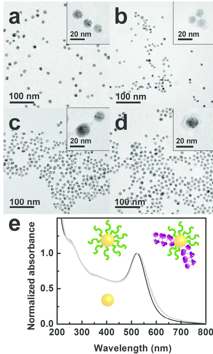
Figure 4. TEM images of (a) Au NPs conjugated with a peptide and exchanged with b) A3cys 3 , c) a2cys 3 and d) a17cys 3 proteins. The insets present the TEM images of the corresponding stained samples. (e) Normalized UV-visible spectra of the samples (a) to (d): in black the as-synthesized Au NPs and in grey, the Au NPs functionalized with a peptide or an aRep protein (all data strictly overlap).
