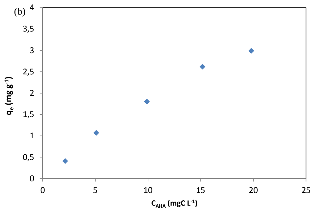
Fig. 8 (b) effect of initial concentration on AHA sorption ( m_{AA} = 0.1 \text{ g} )
