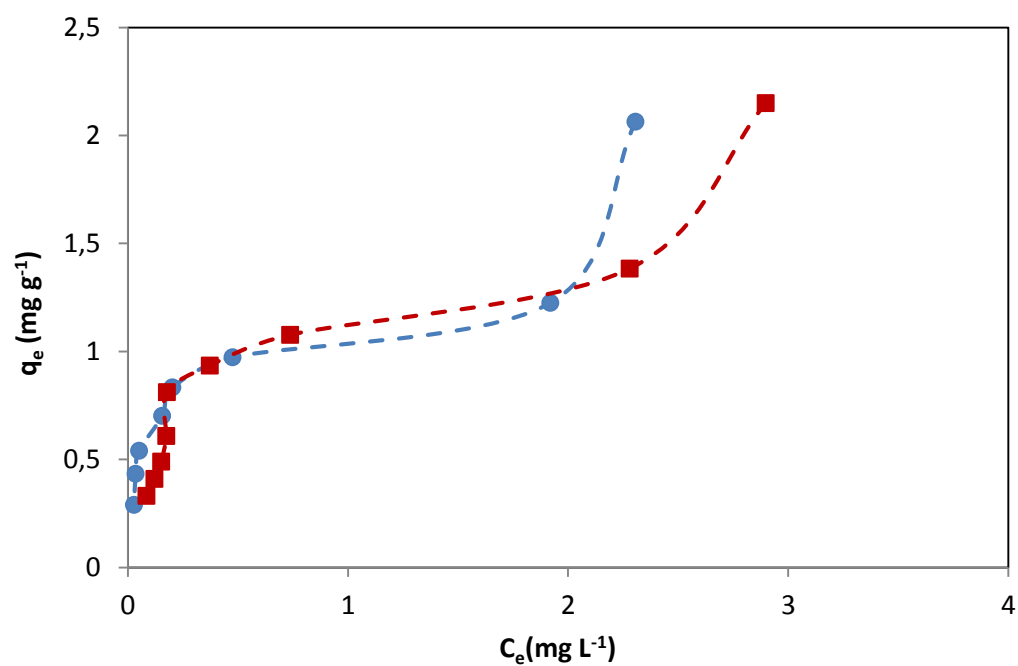
Fig. 10. Fluoride sorption isotherms: in absence of AHA (●) and in the presence of AHA(■) (initial concentration of AHA C_{\text{AHA}} = 5 \text{ mgC L}^{-1} )
