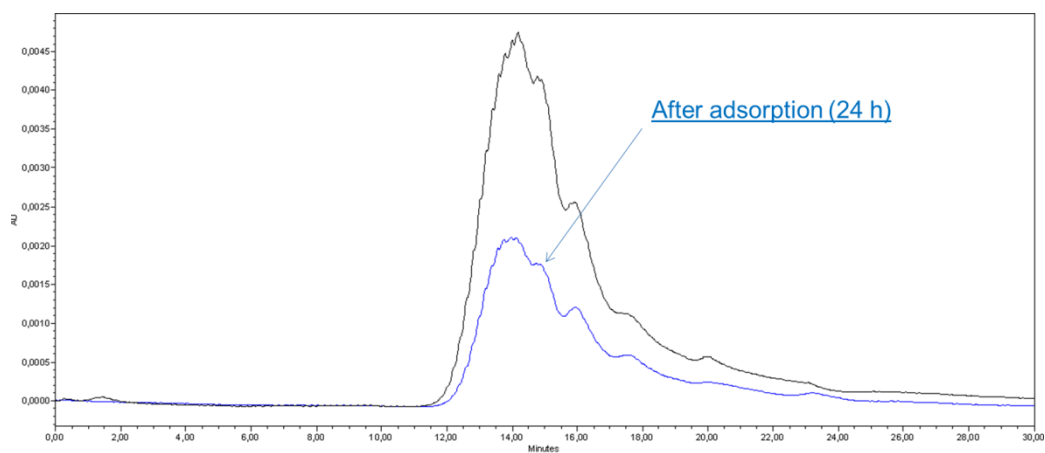
Fig. 7. HPSEC Chromatogram of AHA before and after adsorption onto AA (Operating conditions: V_{inj}=100\text{ }\mu\text{l} ; adsorbent dose= 1\text{ g}_{AA} ; C_{HA}=5\text{ mg L}^{-1} ; T=25\text{ }^{\circ}\text{C} ; Eluant: Sodium Acetate ( 10\text{ mM} , \text{pH}=7 ))
