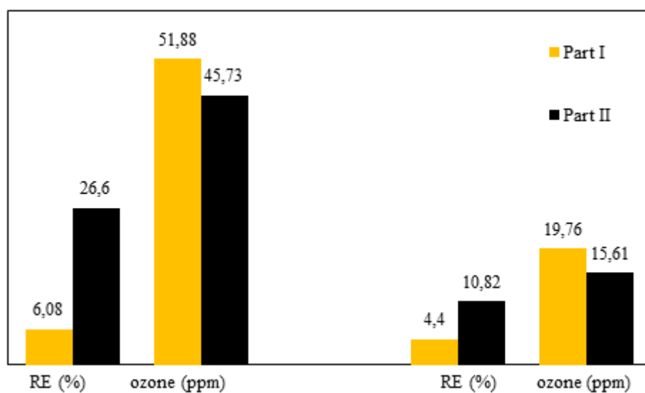
Figure 11. Effect of RH on BUTY conversion rate and ozone formation in PPC for the same BUTY inlet concentration ( Q_{air} = 2 \text{ Nm}^3 \cdot \text{h}^{-1} , [\text{C}_4\text{H}_8\text{O}] = 50 \text{ mg} \cdot \text{Nm}^{-3} , E_{inj} = 12.96 \text{ J} \cdot \text{L}^{-1} , T = 18\text{-}20^\circ\text{C} ) On the left: RH = 5-7 %, On the right: RH = 55 %.
