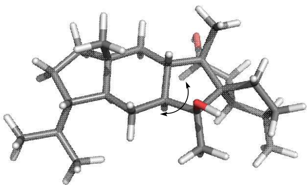
Fig. 3. The optimized conformation of 1 and 2 calculated with DFT/B3LYP/6-31+G(d,p) and NOESY key correlations.
